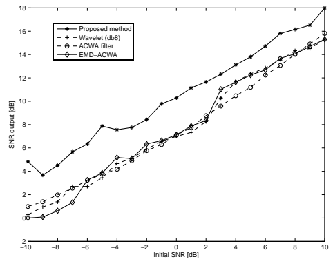
(b) Gain in SNR for noisy version of /a/.
