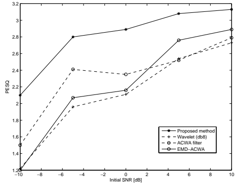
(b) PESQ for noisy version of /a/.
