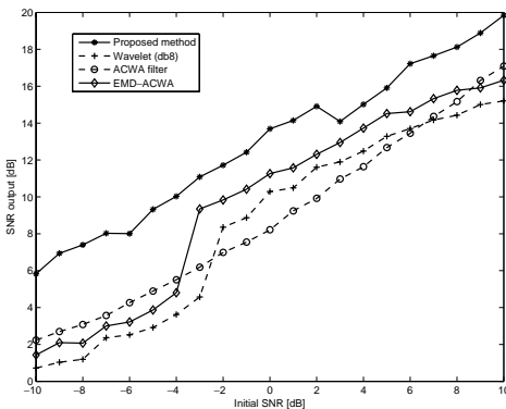
(a) Gain in SNR for noisy version of /o/.
