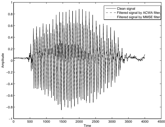
Fig. 1. Clean and filtered signals by the ACWA and the MMSE filters ( \text{SNR}_{\text{in}} = 2 dB).
